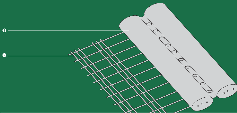
① PVC soft foam (printed) ② reinforced polyester base material
